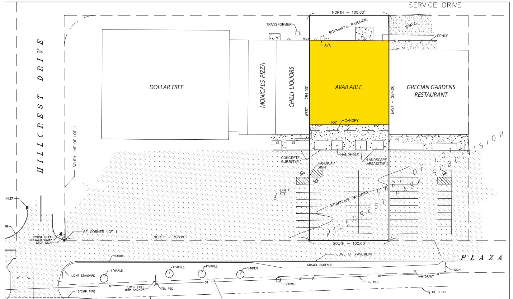
SITE PLAN
